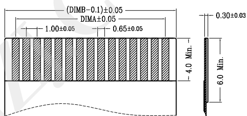
适用扁平线 (Applicable Flat Cable)
